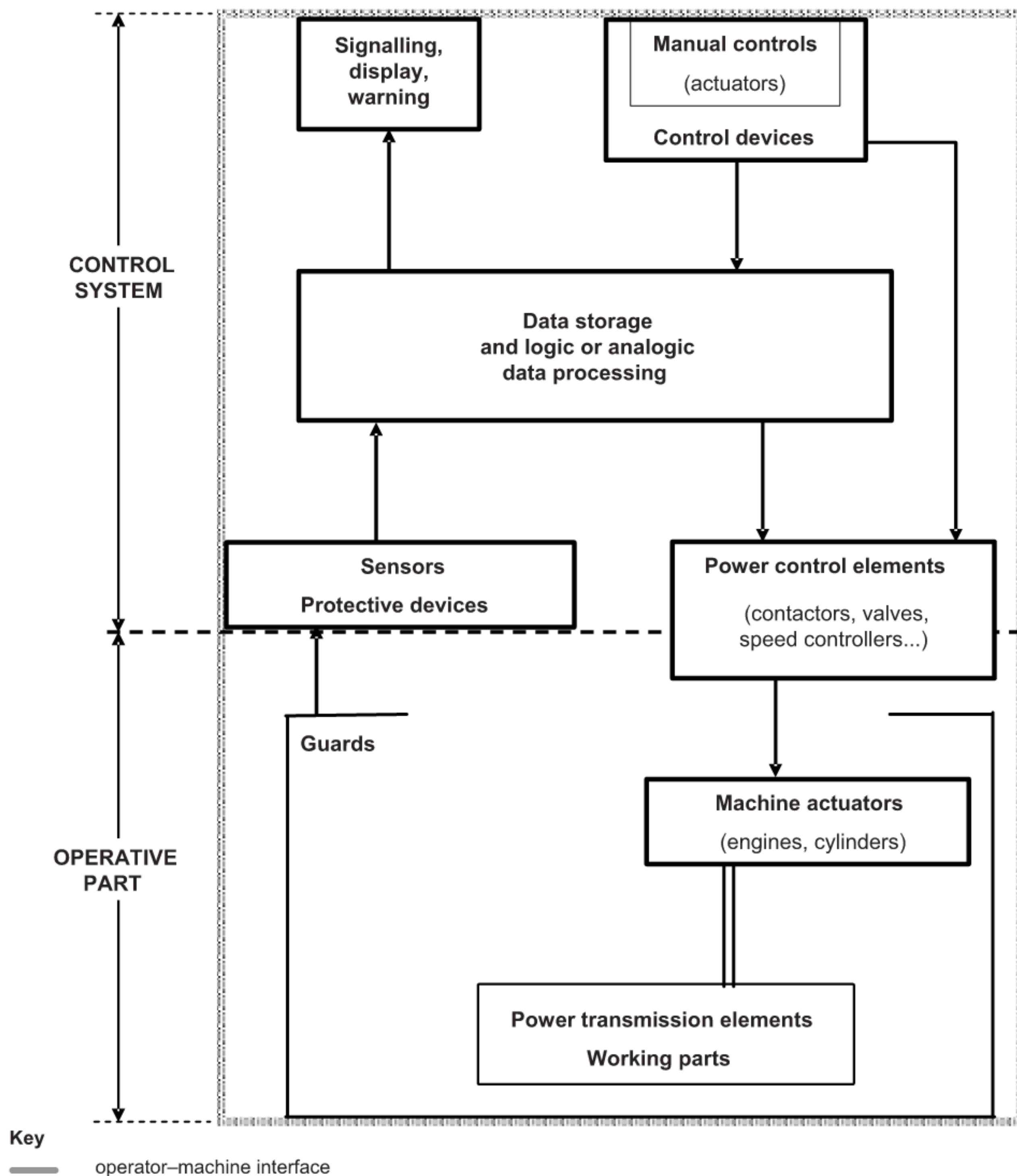
Figure A.1 — Schematic representation of a machine
