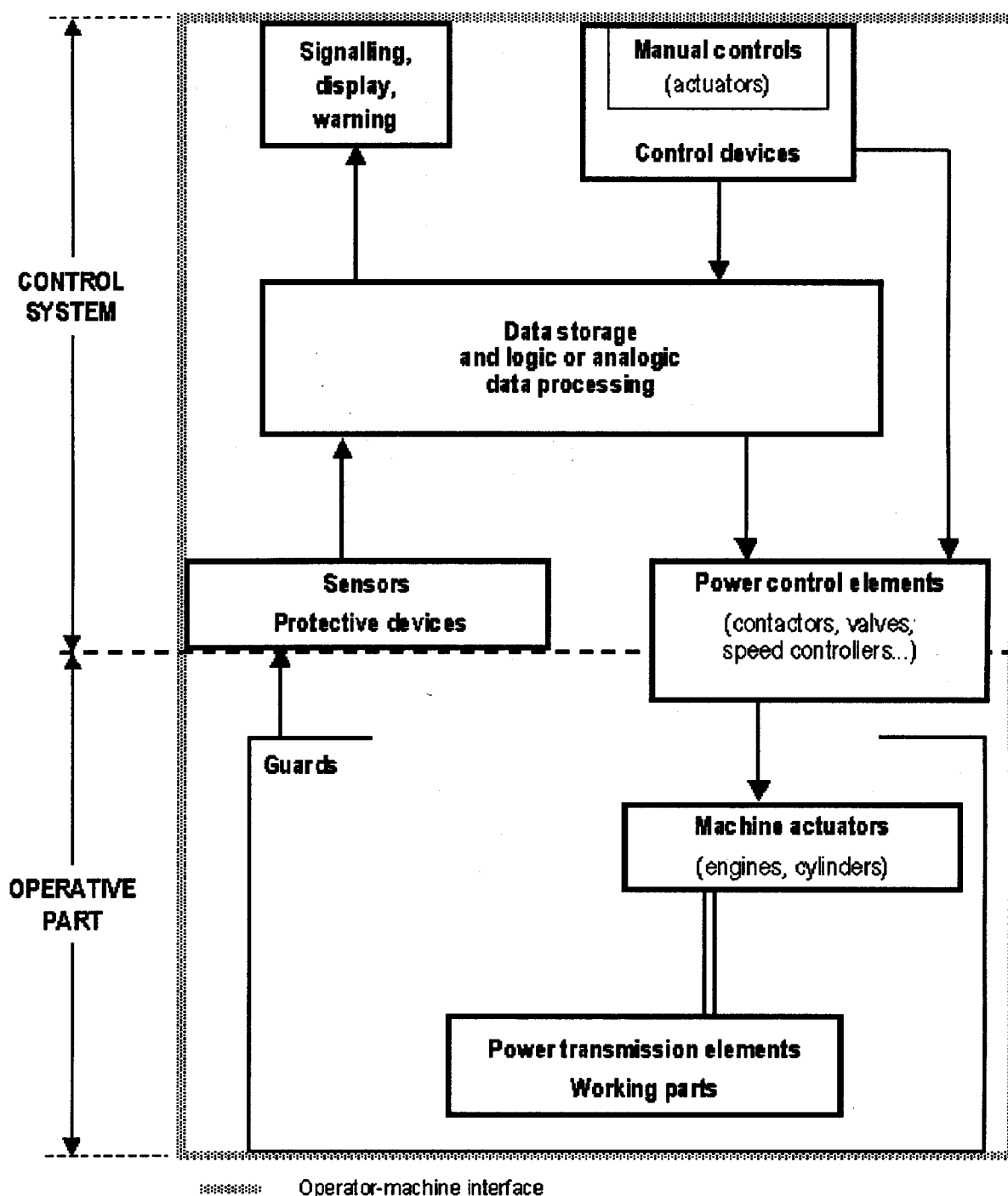
Figure A.1 — Schematic representation of a machine
